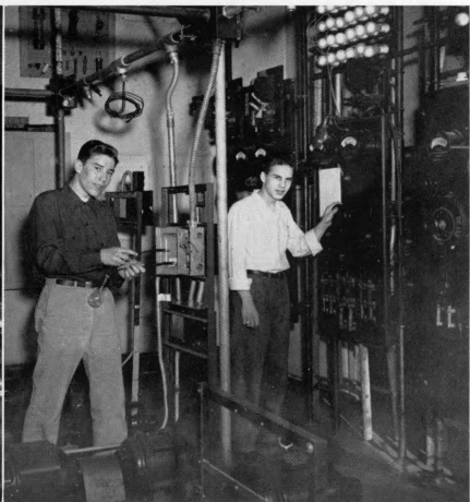
Bob Carlson testing a starting box. John Chaney operating a switchboard as he tests a generator.
